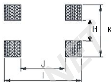
Pad Layout
